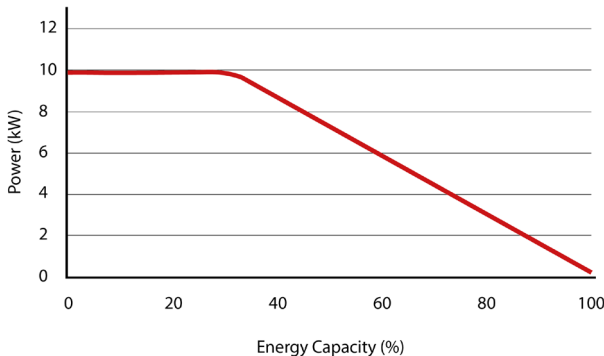
Charge Performance
