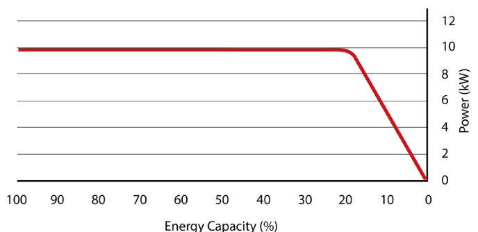
Discharge Performance
