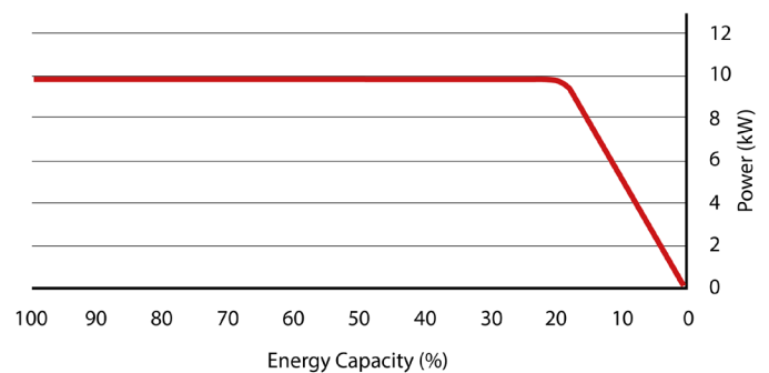
Discharge Performance
