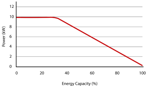
Charge Performance
