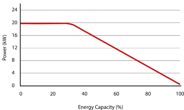
Charge Performance
