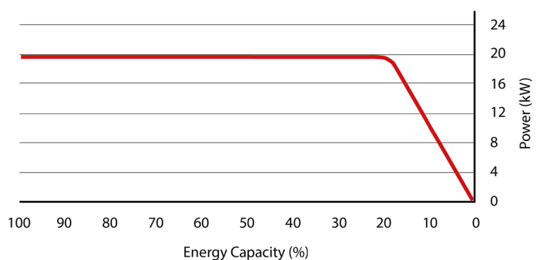
Discharge Performance
