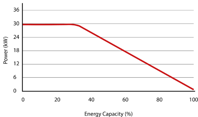
Charge Performance
