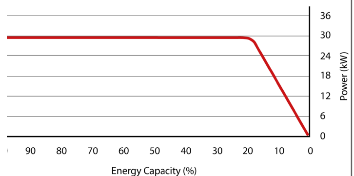
Discharge Performance
